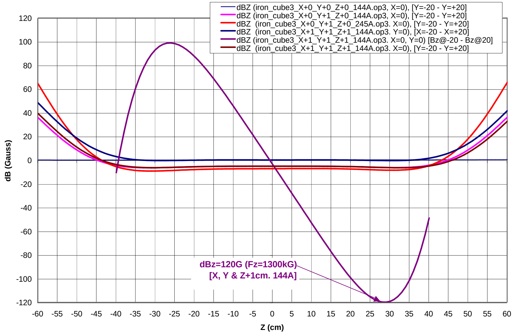
E614_Iron_cube3_X+0_Z+0_***A. X=0. Coils shifted by 0cm or +1cm
