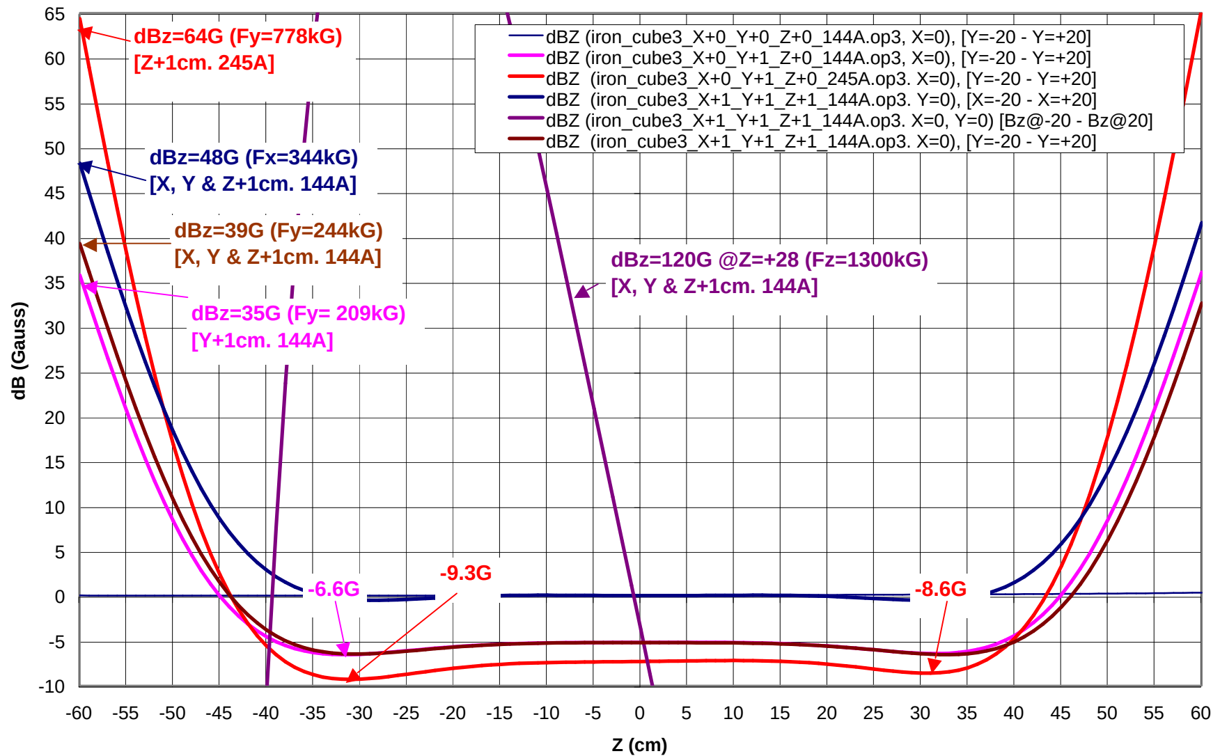
E614_Iron_cube3_X+0_Z+0_***A. X=0. Coils shifted by 0cm or +1cm
