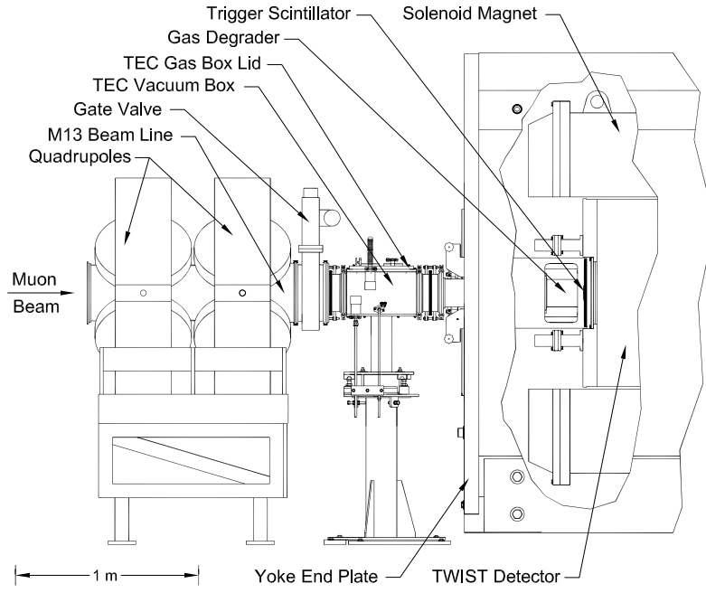
Figure 2.4: Positioning of the time expansion chambers relative to the M13 beam line and solenoid[76].
