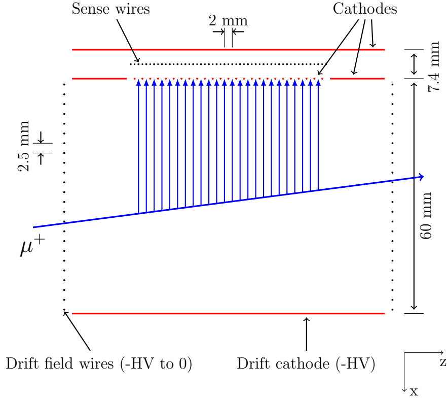
(a) Components of a single time expansion module[76].
