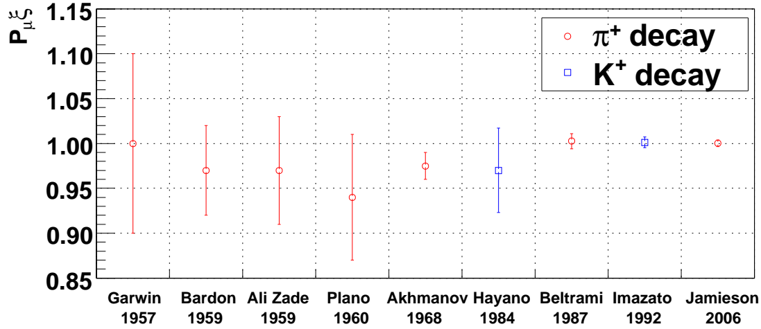
Figure 1.5: Previous direct measurements of P_\mu\xi with uncertainties less than 10%. The statistical and systematic uncertainties have been added in quadrature. Measurements are from Refs [21, 62, 64, 65, 66, 67, 68, 69, 70].
