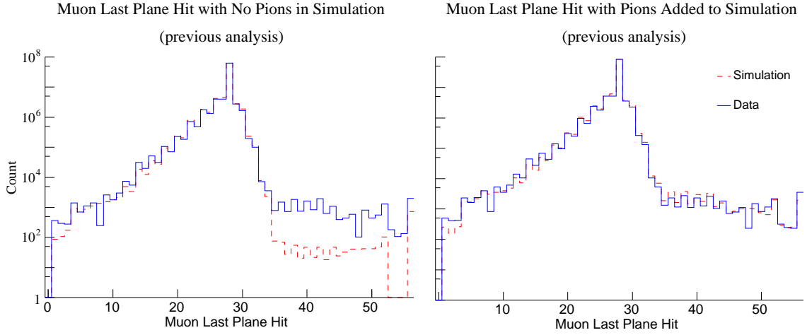
(a) Distribution of last plane that measures the muon, for data and simulation, from the previous analysis (originally Fig. 6.9 from Ref. [57]). The mismatch is resolved by including an additional source of pion decays at the location of the upstream beam package.
