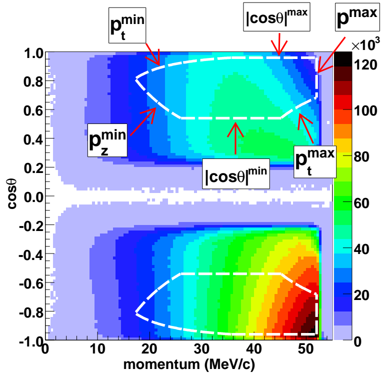
(c) Reconstructed spectrum with fiducial boundaries.
