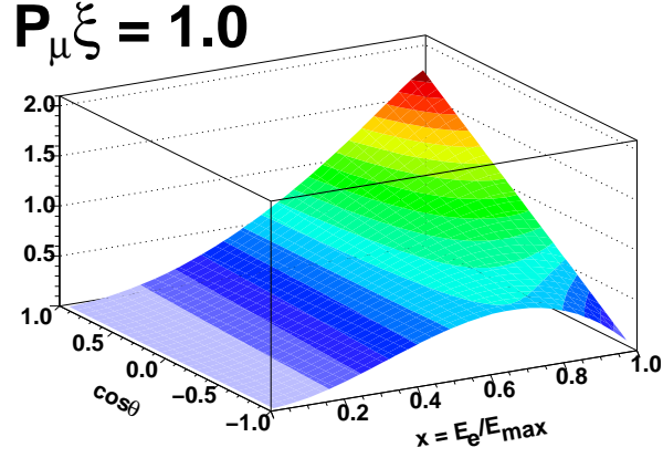
(a) Standard model, P_\mu^\pi \xi = 1 .
