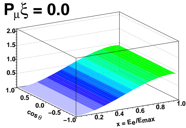
(c) P_\mu^\pi \xi = 0
