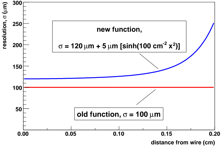
Figure 3.8: Resolution function used during the helix fitting.
