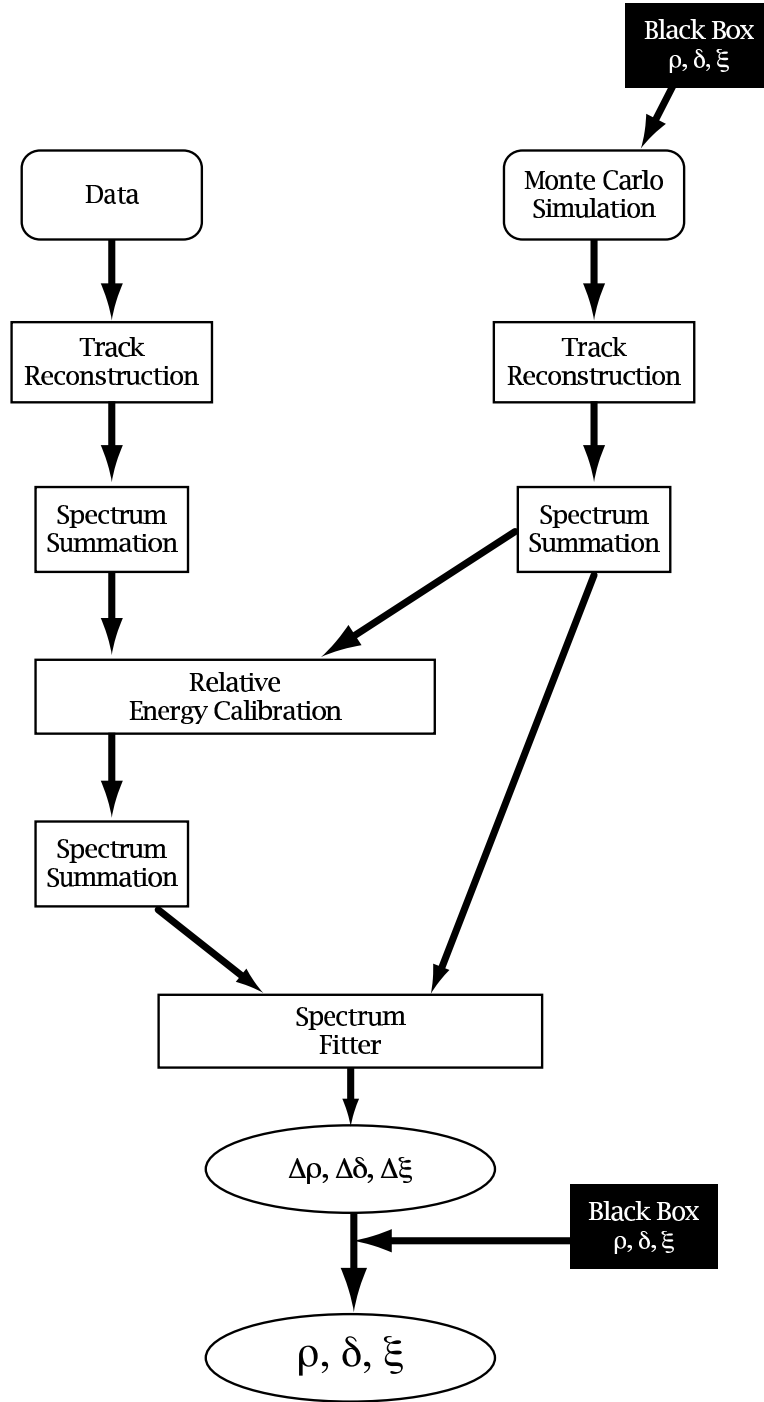
Figure 3.1: Flow diagram of the analysis procedure[83]. The “Black Box” corresponds to the hidden values of the muon decay parameters.
