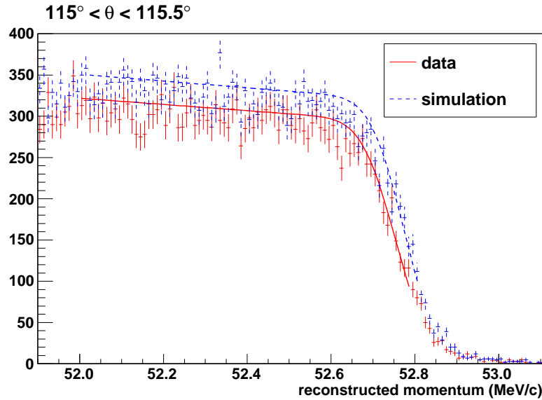
Figure 3.14: Example of the kinematic endpoint in data and simulation, over a limited angular range.
