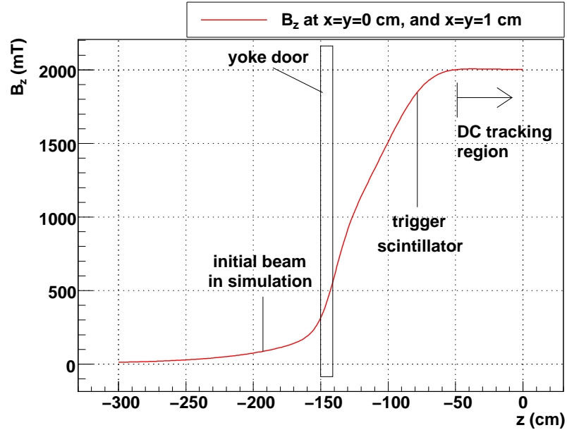
Figure 6.2: Longitudinal ( B_z ) components from the field map used for the analysis. These are produced from an Opera finite element analysis[85].
