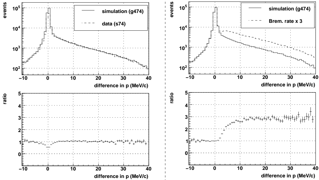
Figure 6.18: The left hand side shows the energy difference for the two halves of a broken track, for data and simulation. The right hand side shows the same distribution for a simulation where the Bremsstrahlung rate was increased by a factor of three. The range ( 15 < p < 35 ) MeV/c is used to evaluate the systematic uncertainty.
