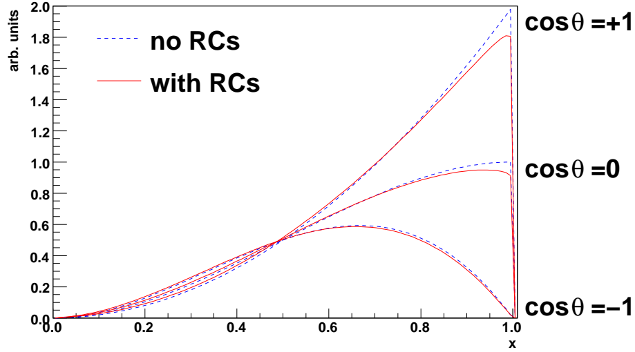
Figure 1.3: Slices of spectrum, demonstrating the effect of radiative corrections (RCs), which are as large as 10% at the maximum positron energy.
