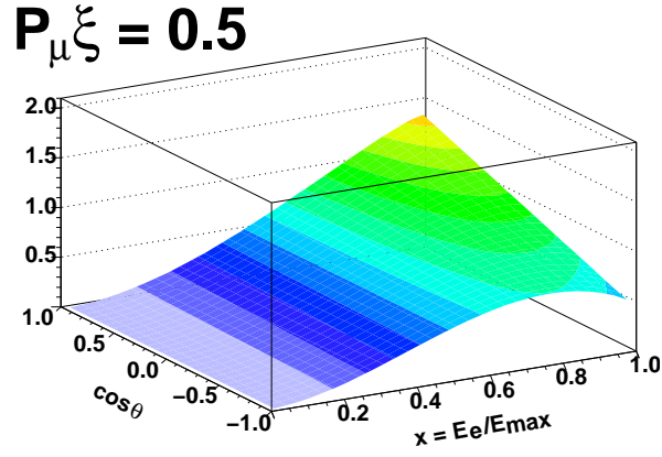
(b) P_\mu^\pi \xi = 0.5
