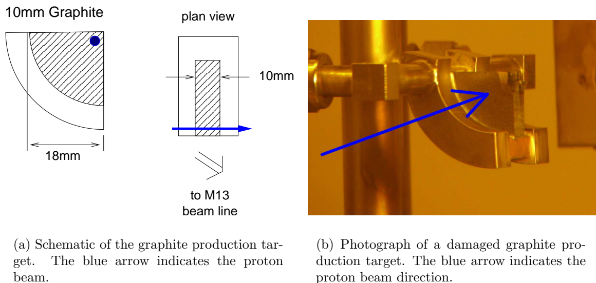
Figure 2.1: Schematic and photograph of a graphite production target.
