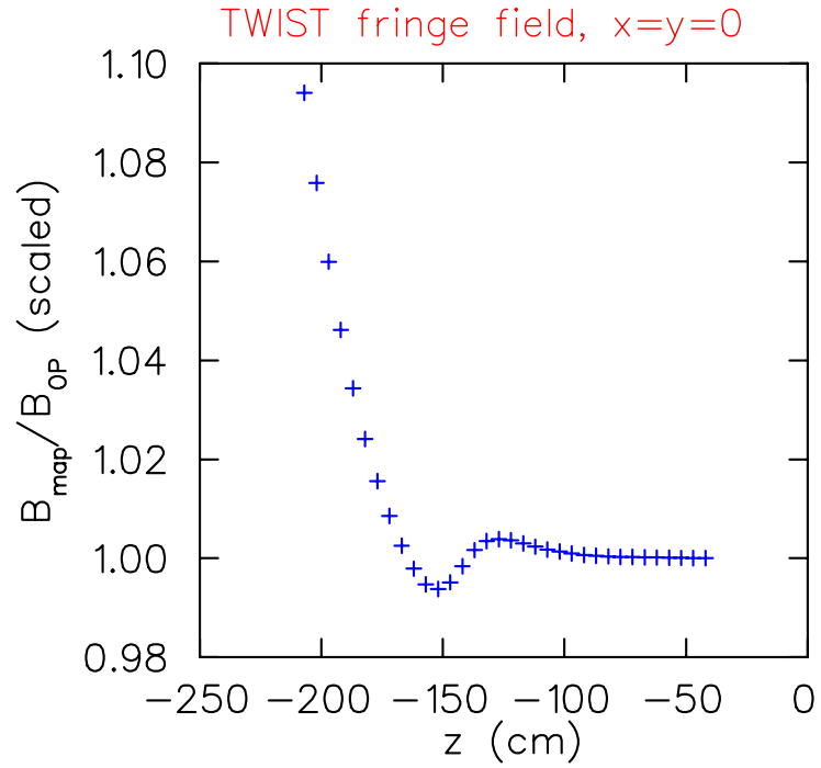
Figure D.4: For x = y = 0 , the ratio of the measured field map to the Opera model[98].
