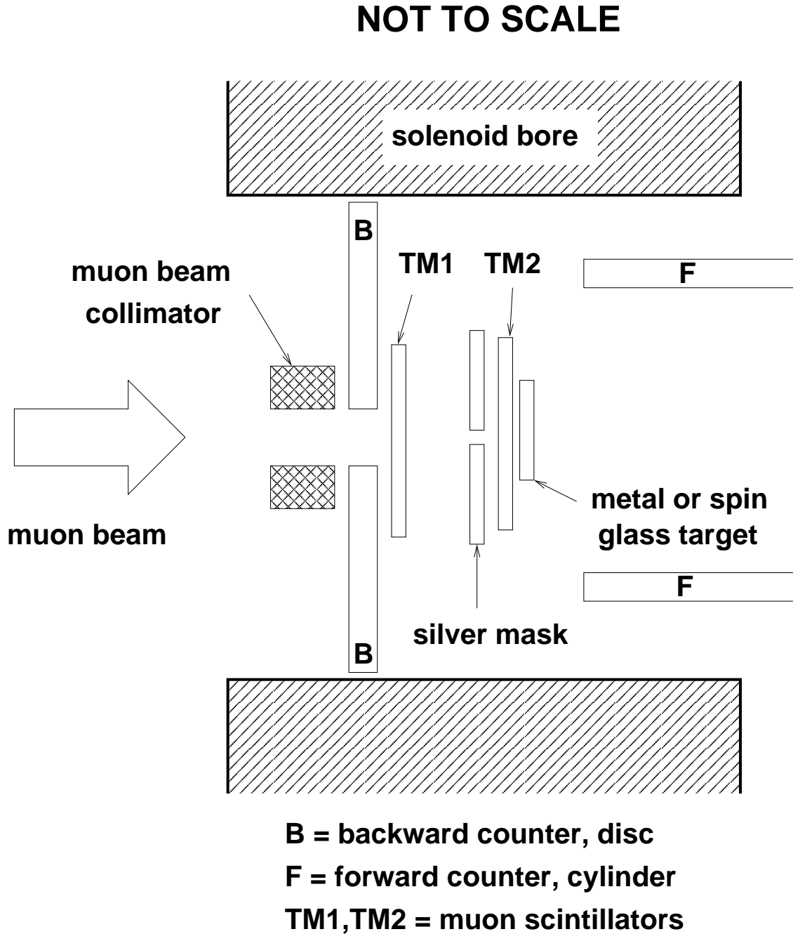
Figure H.1: Schematic for the experimental setup. The muons enter from the left and will trigger an event if they pass through the first scintillator (TM1) and stop in the silver mask, or pass through both scintillators (TM1 and TM2) and stop in the target. The backward positron counter (B) is protected from the muon beam by a collimator. Materials such as the beam pipe, beam line windows, vacuum tubes, light guides, and cryostat are not shown.
