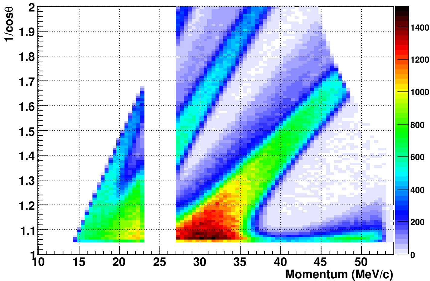
US Spectrum (after cuts), Data
