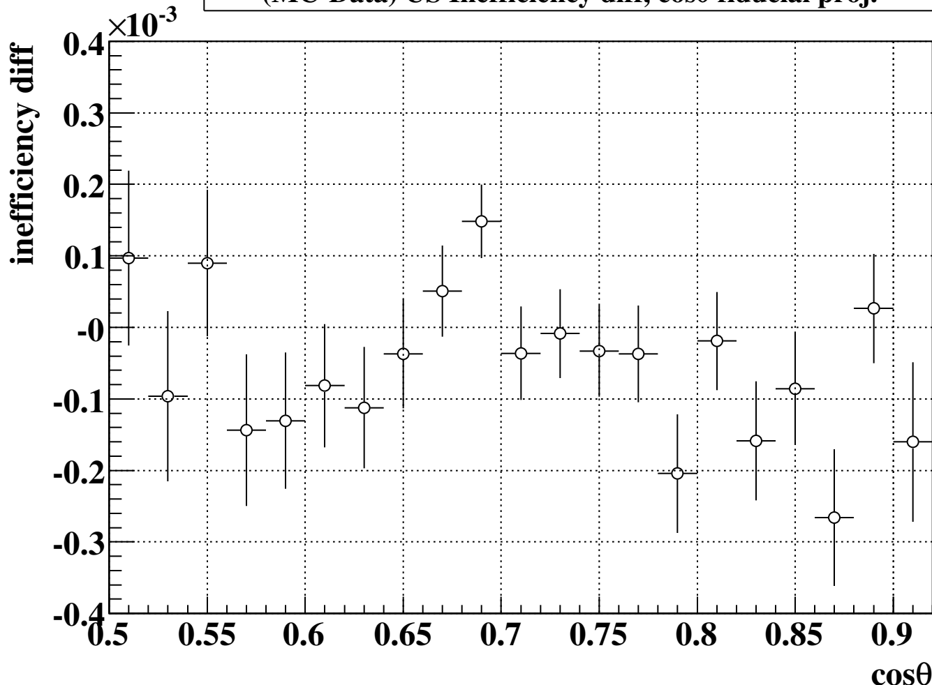
(MC-Data) US Inefficiency diff, \cos\theta fiducial proj.
