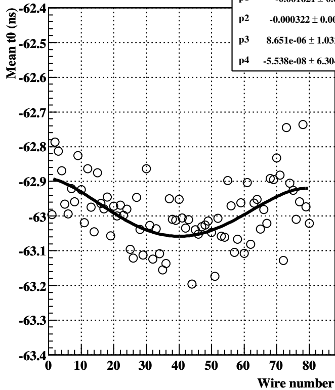
Average t0, DS V planes, MC
