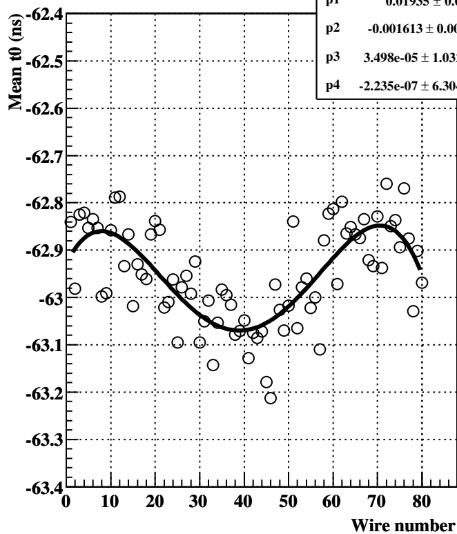
Average t0, US V planes, MC
