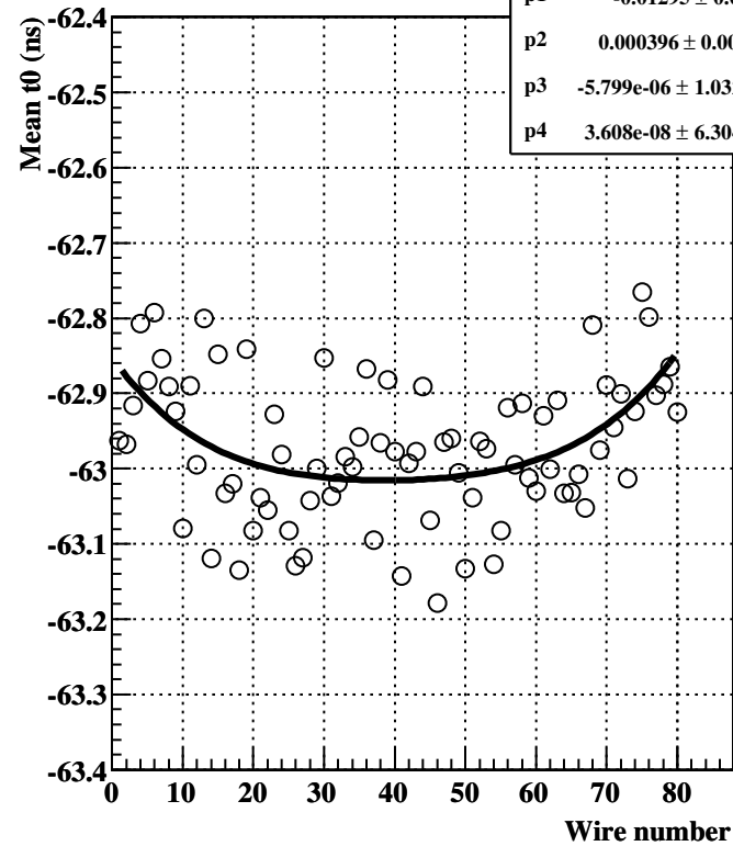
Average t0, DS U planes, MC
