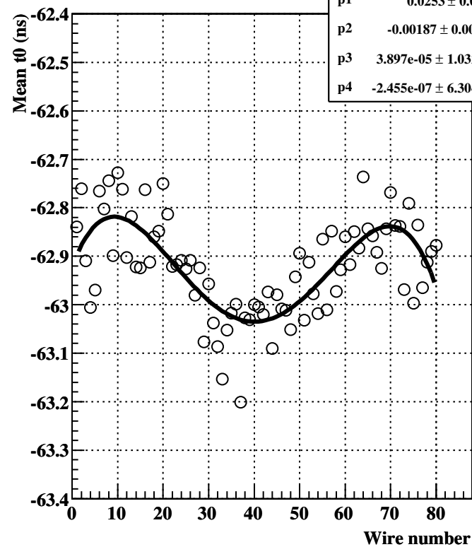
Average t0, US U planes, MC
