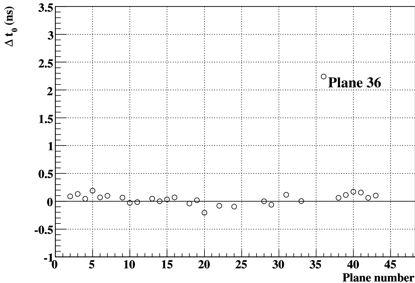
(End-Start) \Delta t_0 plane averages
