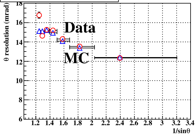
\theta resolution, p=32.5 MeV
