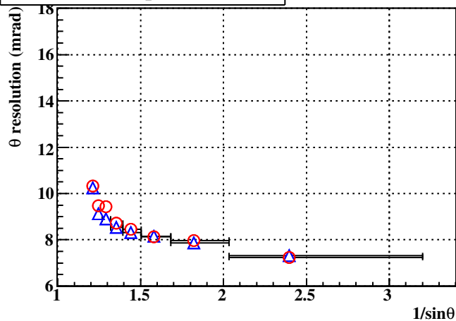
\theta resolution, p=37.5 MeV
