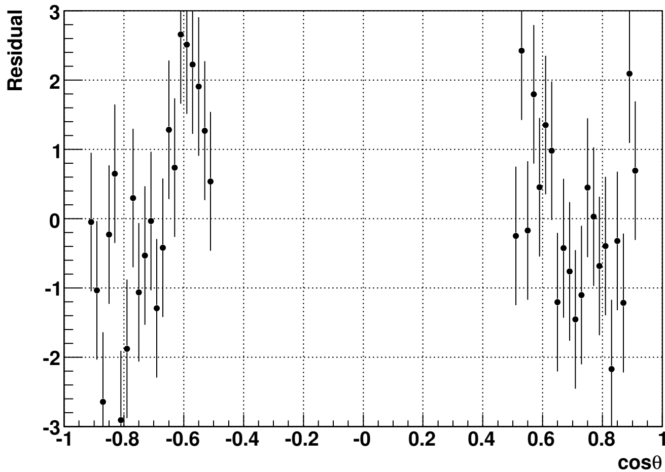
Fit residuals (Data-Fit)/ \sigma , fiducial region only
