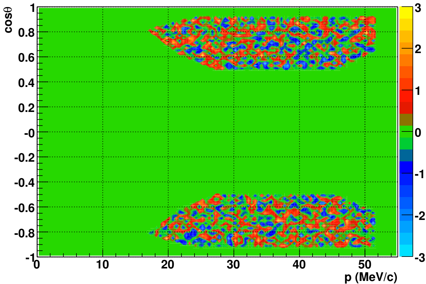
Fit residuals, Bremsstrahlung rate \times 3
