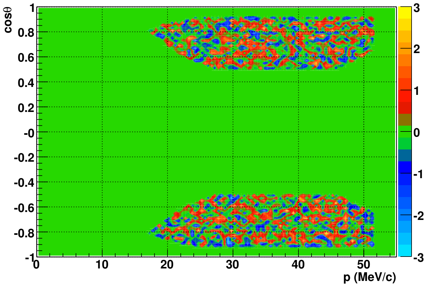
Fit residuals, \Delta \text{ray rate} \times 3
