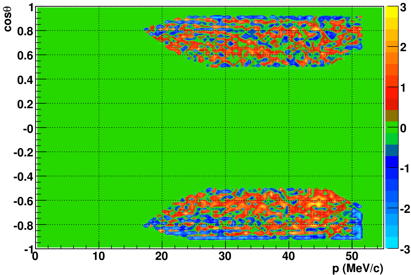
Fit residuals, delta ray rate \times 10
