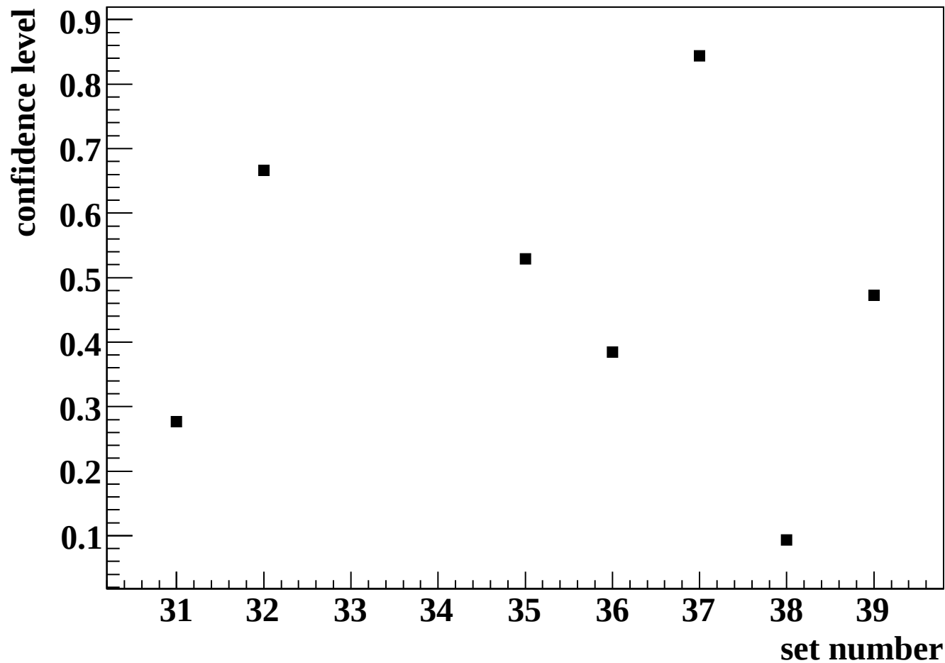
Confidence level for Michel spectrum fits
