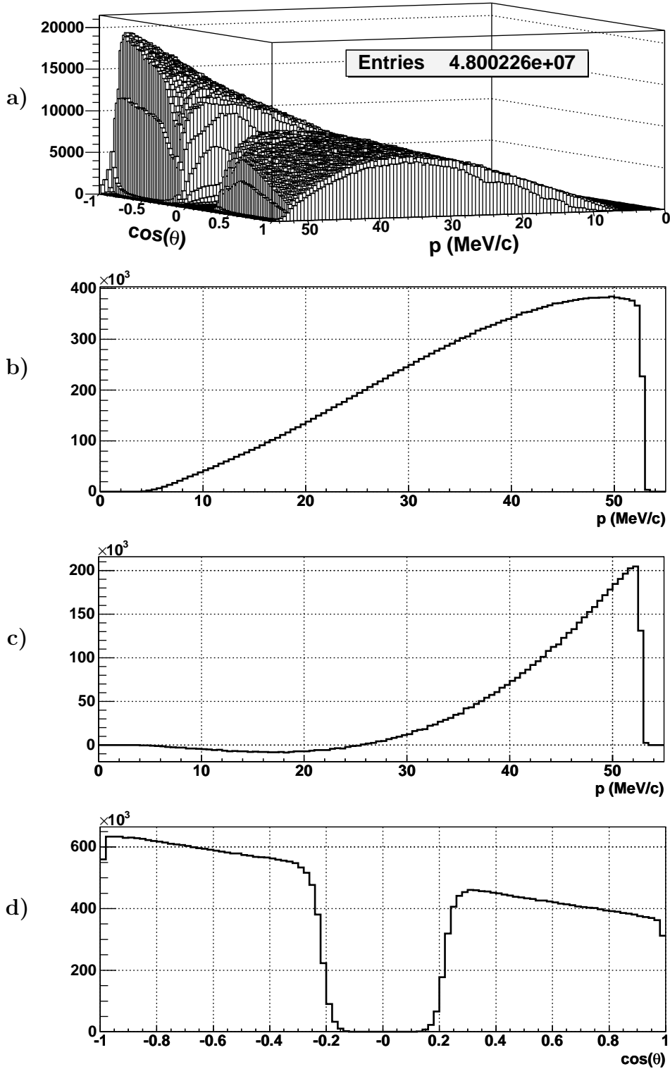
Figure 5.3: Reconstructed data spectrum from set B. a) In the momentum- \cos(\theta) plane. b) Momentum spectrum for 0.50 < |\cos(\theta)| < 0.84 , proportional to F_{IS}(p) . c) Difference of momentum spectra for -0.84 < \cos(\theta) < -0.50 and 0.50 < \cos(\theta) < 0.84 , proportional to F_{AS}(p) d) \cos(\theta) spectrum for 20 < p < 50 MeV/c.
