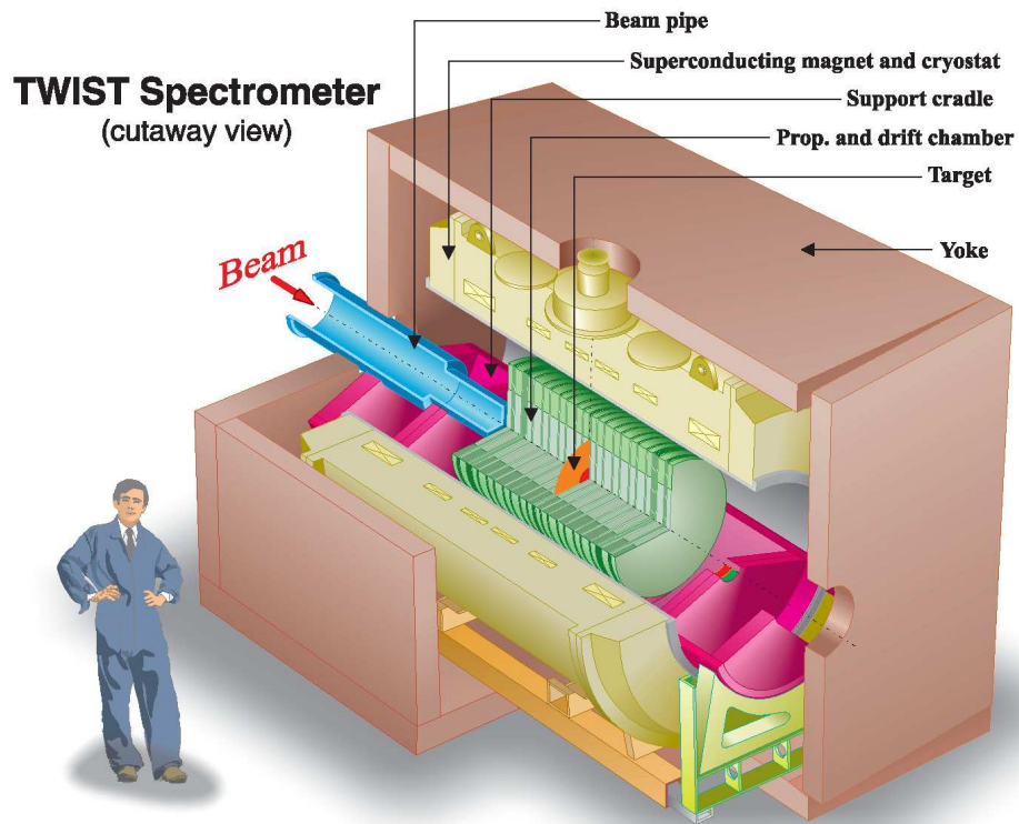
Figure 2.1: A drawing of the TWIST detector [52].
