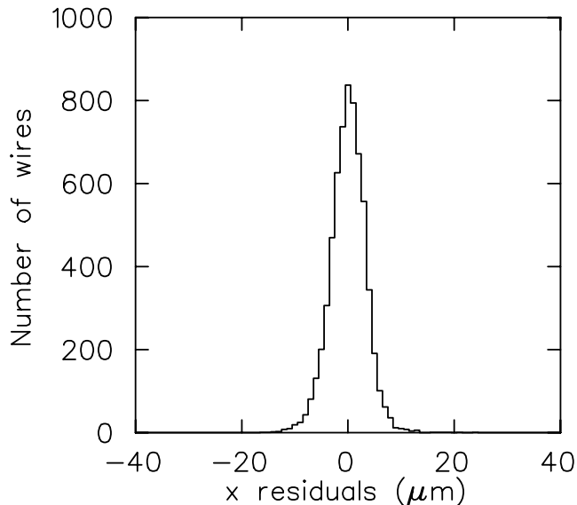
Figure 2.4: Deviation of wires from their nominal positions. \sigma = 3.3 \mu\text{m} [52].
