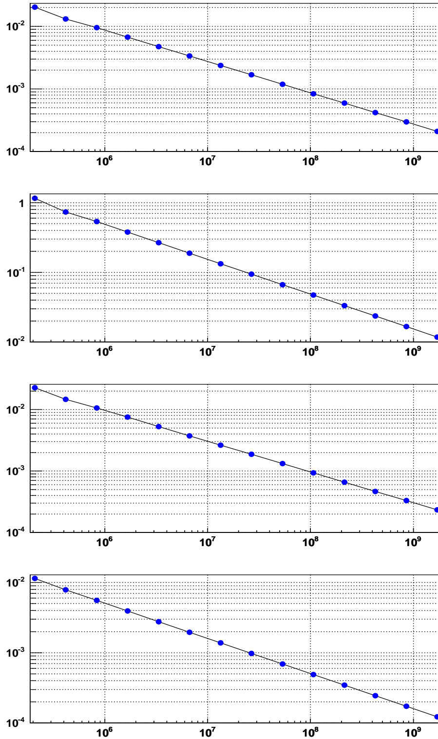
Figure 7.2: Scaling of fit errors with statistics. Horizontal axis: the number of data events in the fiducial region. Vertical axis: the mean value of reported fit error of 18 fits at the given statistics. Top to bottom: \rho , \eta , P_\mu \xi , \delta .
