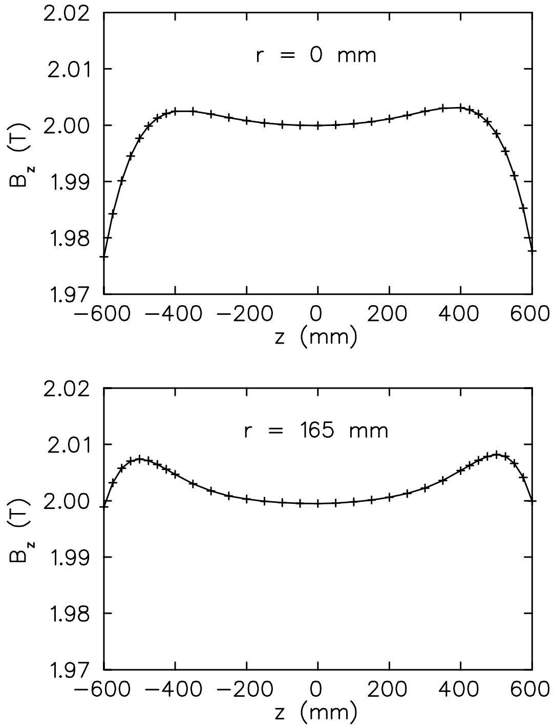
Figure 2.5: B_z vs z on the detector axis (top), and at the edge of the tracking volume (bottom). Note the zoomed vertical scale. The limits of the tracking volume in z , defined by the outermost DCs, are \pm 500 mm. The radius of the tracking volume is defined by the size of the wire planes. Plots from [57].
