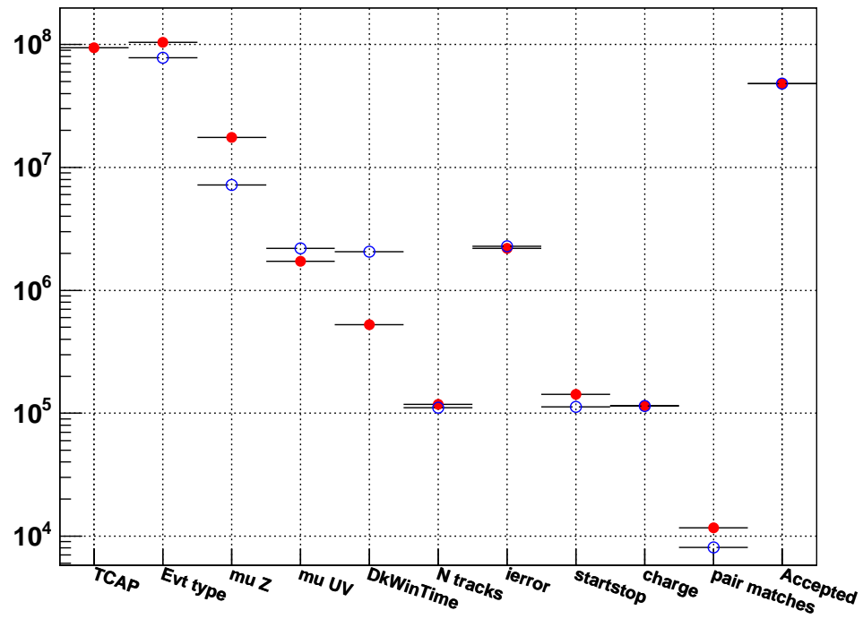
Figure 5.1: Top: each bin contains the number of events before the cut; bottom: the number of events rejected by cut. Solid markers: data, empty markers: MC. Monte-Carlo is normalized to data by matching the number of accepted events.
