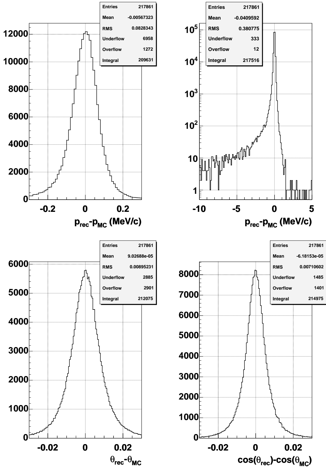
Figure 5.4: Distributions of differences of reconstructed and Monte-Carlo values. Top row: momentum, on different scales. Bottom left: \theta , bottom right: \cos(\theta) .
