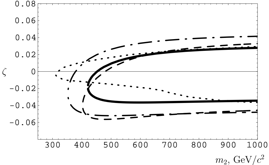
Figure 10.1: 90% CL constraints on manifest left-right symmetric models. The excluded region is low mass and large |\zeta| . Bold line: TWIST lower limit on P_\mu\xi . Dashed line: dedicated search for right-handed currents in muon decay [100]. Dash-dotted line: one-sided limit P_\mu\xi > 0.991867 (90% CL) from a direct measurement of P_\mu\xi [104]. Dotted line: combined nuclear beta decay data [103].
