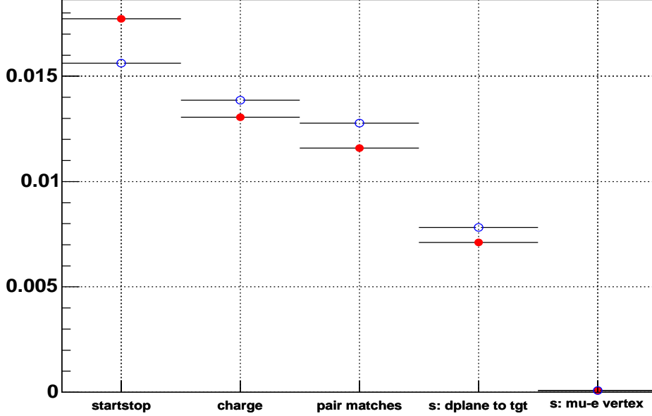
Figure 5.2: The mean number of extra decay track candidates before cut or select. Solid markers: data, empty markers: MC.
