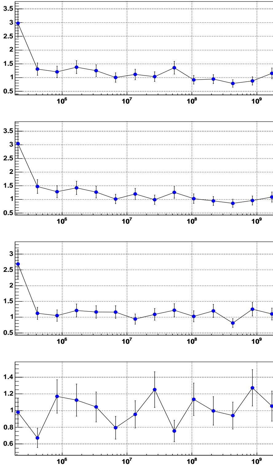
Figure 7.4: The reliability of fit error estimate as function of statistics. Horizontal axis: the number of data events in the fiducial region. Vertical axis: RMS/(Mean fit error) of the 18 fits at the given statistics. Top to bottom: \rho , \eta , P_\mu \xi , \delta .
