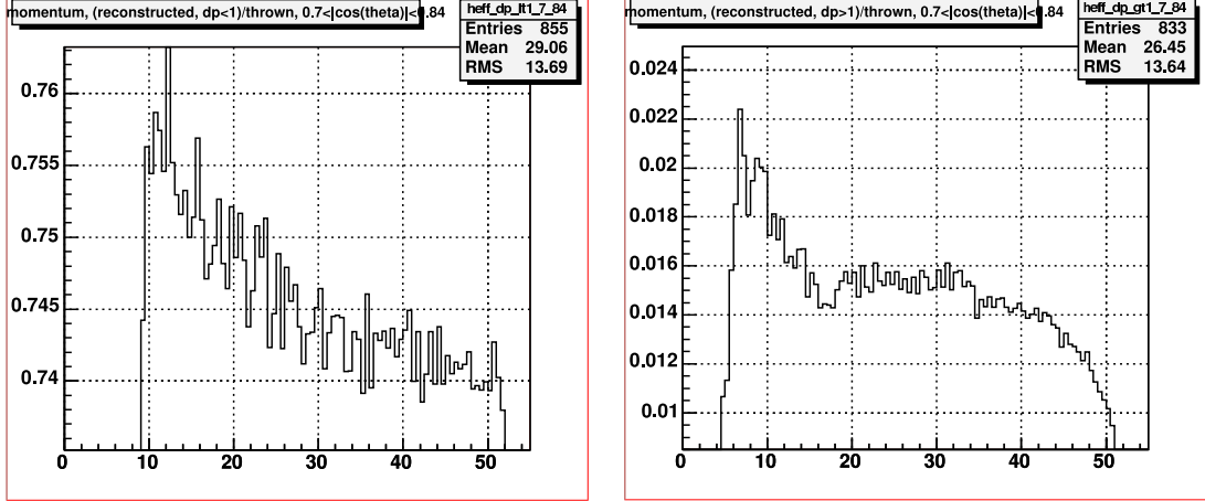
Figure 8.1: Ratios of (reconstructed)/(thrown) momentum spectra for: \Delta p_{MC} \leq 1 MeV/c (left), \Delta p_{MC} > 1 MeV/c (right). Only events with 0.7 < |\cos(\theta)| < 0.84 are included in the spectra. (Plots from [90].)
