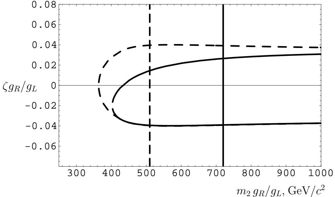
Figure 10.2: A comparison of model dependence of muon decay and collider limits on left-right symmetric models. Solid lines: 95% CL limits on manifest left-right symmetry from TWIST (curved line) and D0 [108] (vertical). Dashed lines: TWIST exclusion for arbitrary CP violation and right-handed CKM matrices (curved), D0 mass limit for a specific set of parameters of non-manifest model (vertical).
