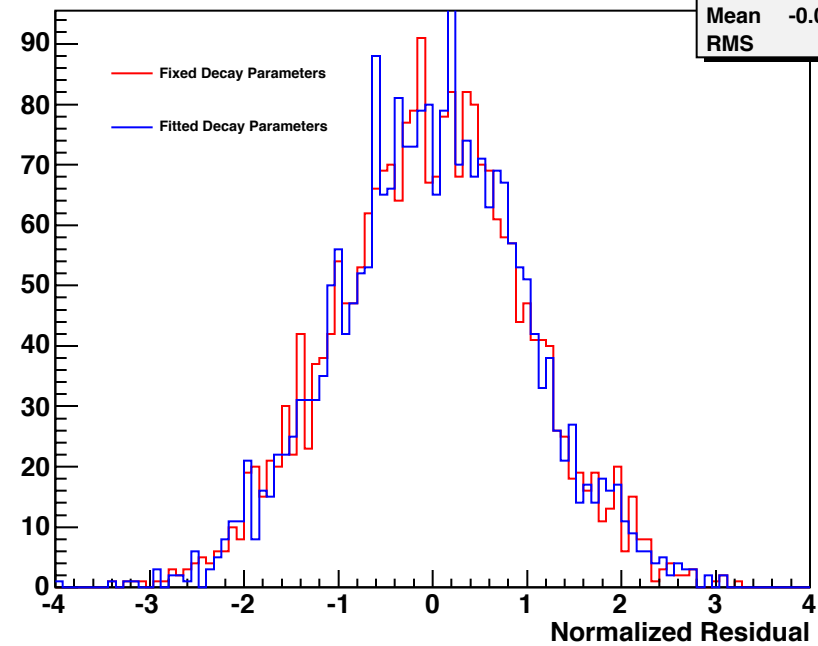
sum71-3-1_sum471-1_21-1_michel.root
