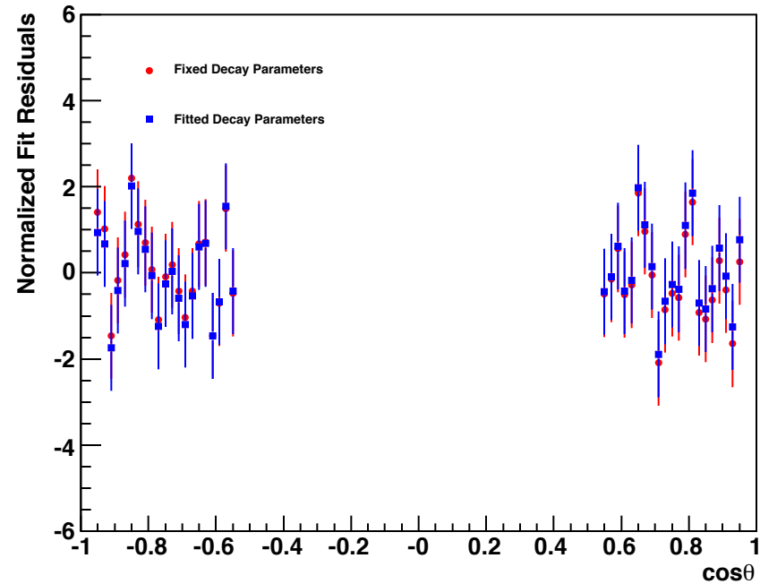
sum74-4-1_sum474-1_2_21-1_michel.root
