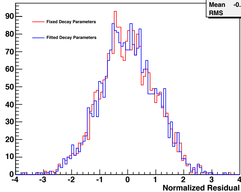
sum70-3-1_sum470-1_21-1_michel.root
