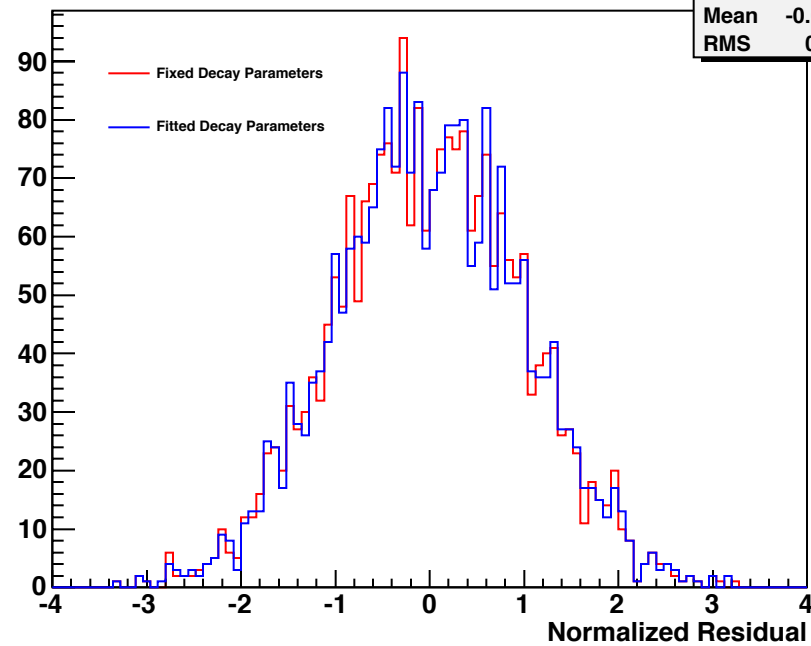
sum83-4-1_sum583-1_2_21-1_michel.root
