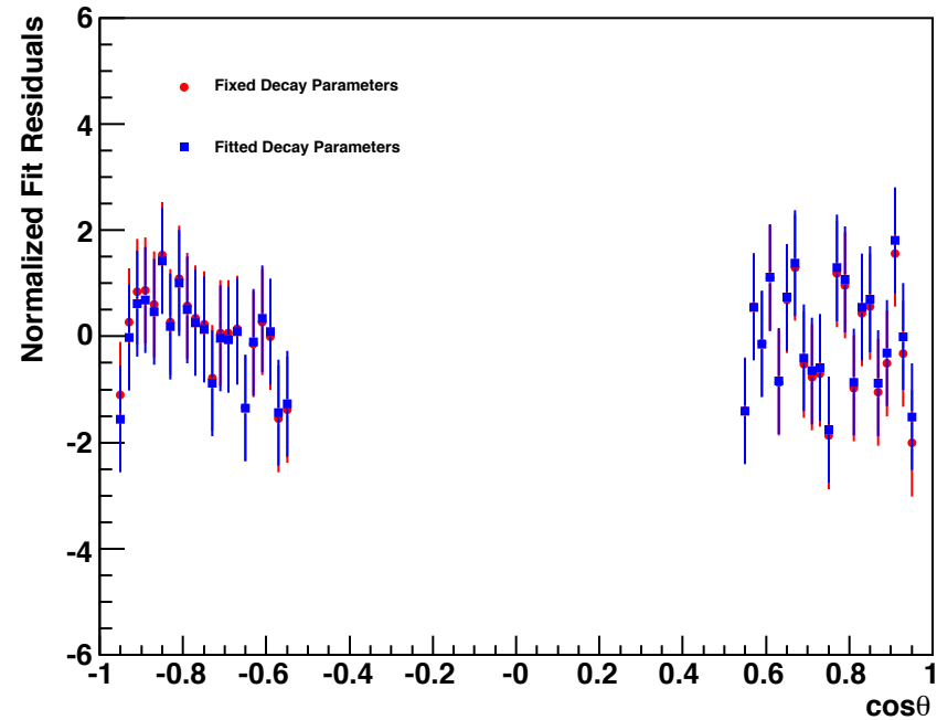
sum70-3-1_sum470-1_21-1_michel.root
