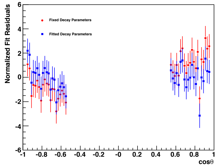
sum76-6-1_sum476-1_21-1_michel.root
