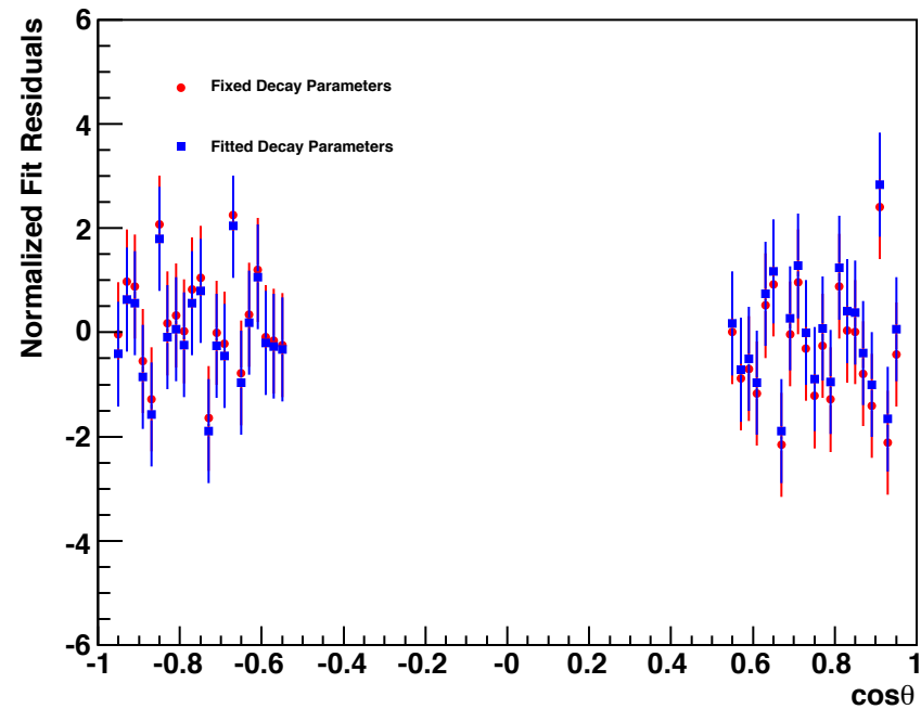
sum68-3-1_sum468-1_21-1_michel.root
