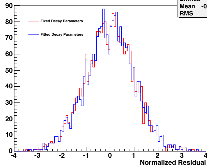
sum72-2-1_sum472-1_21-1_michel.root
