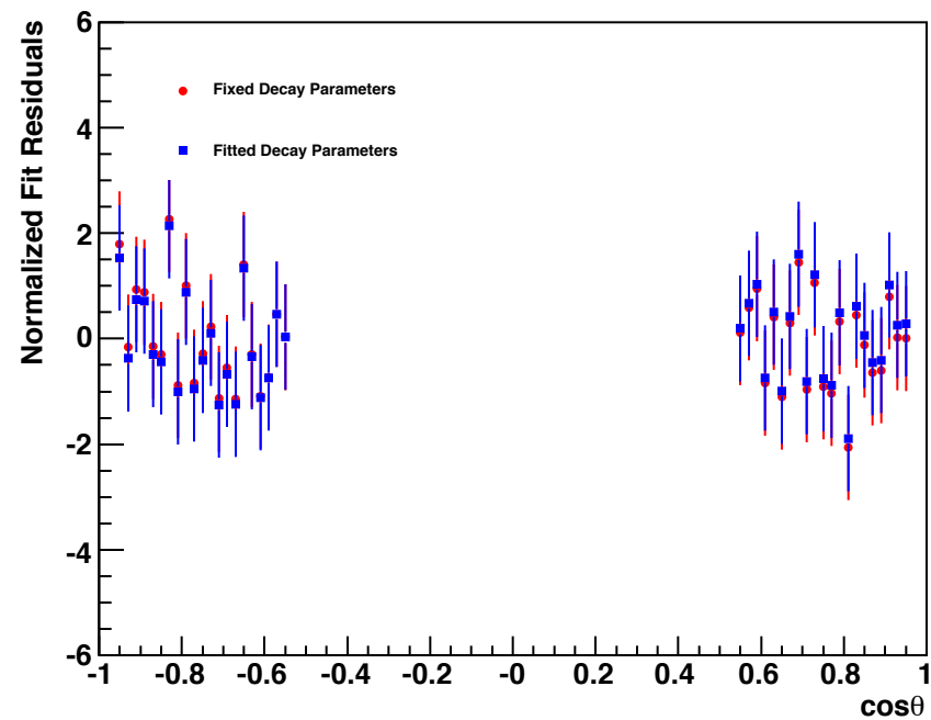
sum87-3-1_sum587-1_21-1_michel.root
