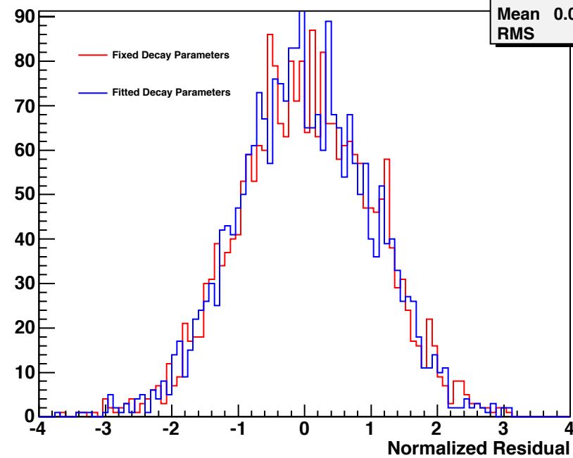
sum76-6-1_sum476-1_21-1_michel.root
