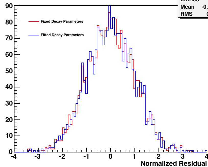
sum87-3-1_sum587-1_21-1_michel.root
