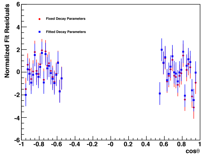
sum75-14-1_sum475-1_21-1_michel.root
