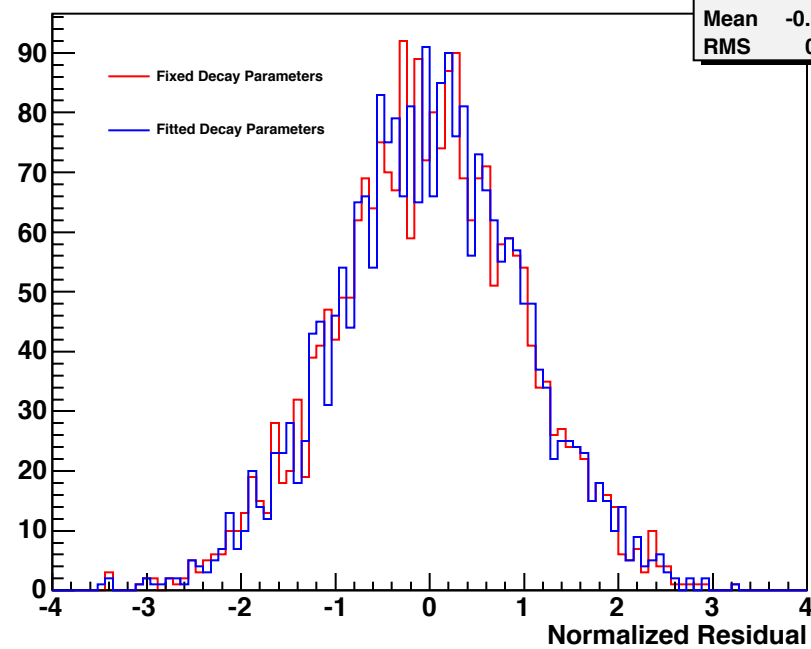
sum68-3-1_sum468-1_21-1_michel.root
