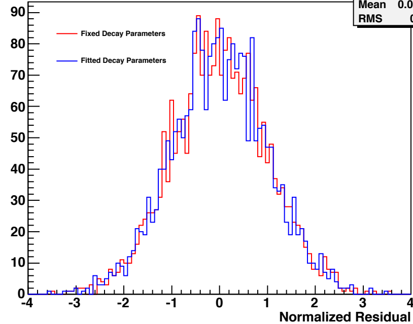
sum86-3-1_sum586-1_21-1_michel.root
