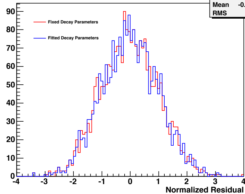
sum74-4-1_sum474-1_2_21-1_michel.root
