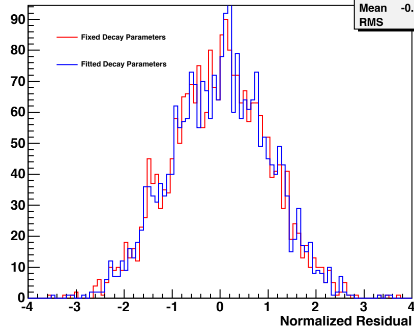
sum75-14-1_sum475-1_21-1_michel.root
