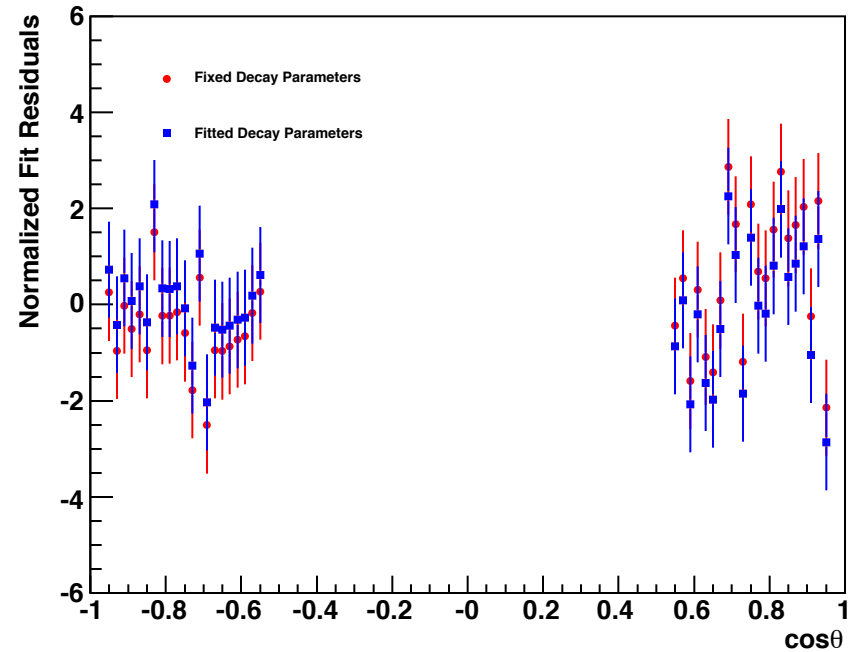
sum86-3-1_sum586-1_21-1_michel.root
