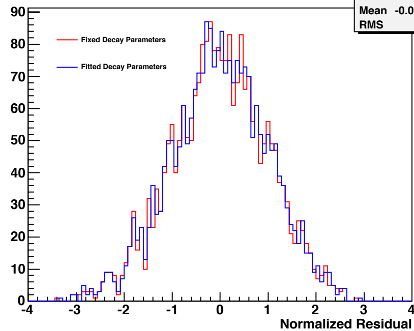
sum92-2-1_sum592-1_21-1_michel.root
