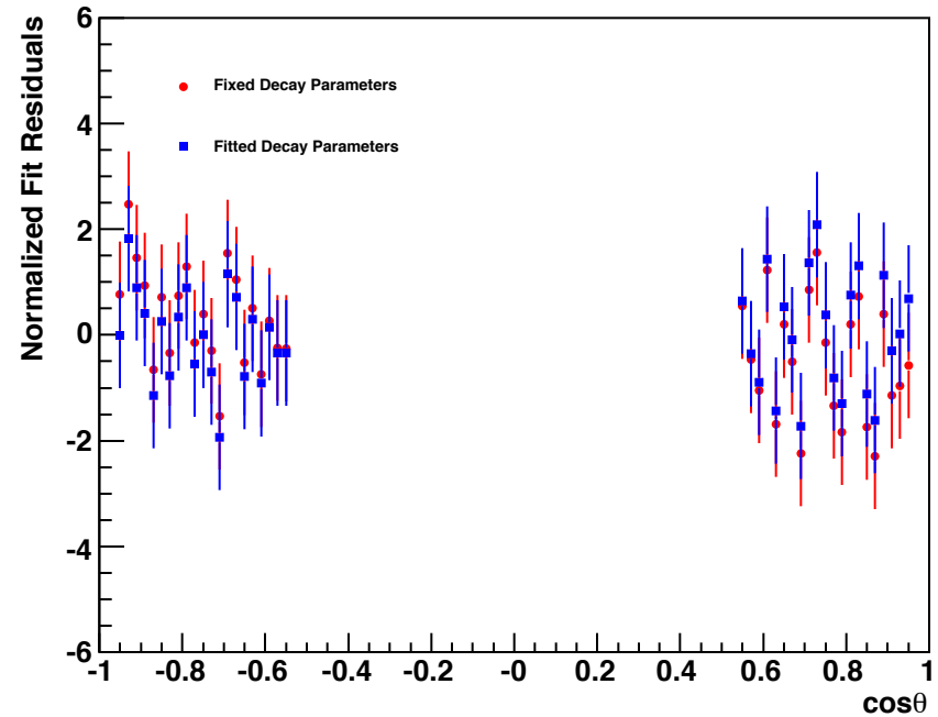
sum71-3-1_sum471-1_21-1_michel.root
