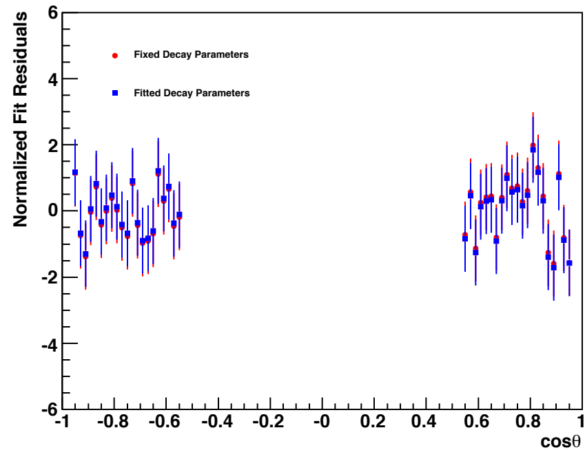
sum92-2-1_sum592-1_21-1_michel.root
