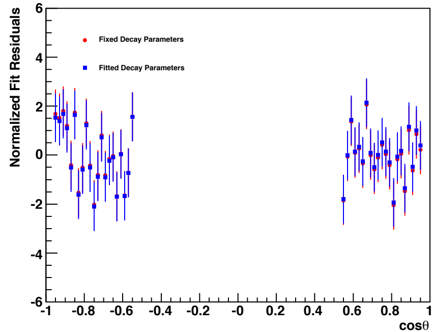
sum83-4-1_sum583-1_2_21-1_michel.root
