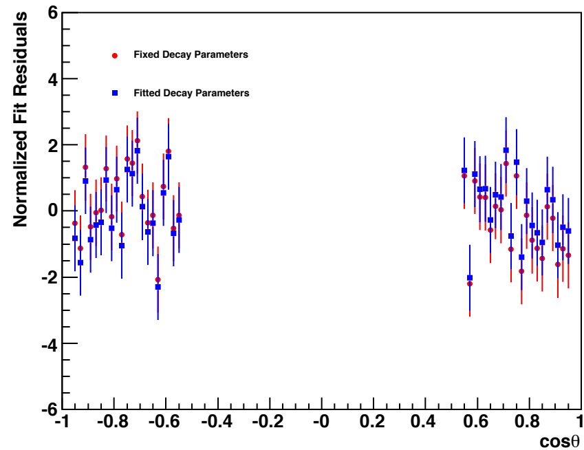
sum72-2-1_sum472-1_21-1_michel.root
