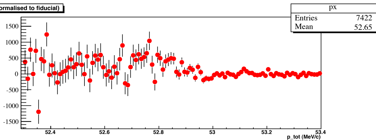
Distribution of Endpoint residuals, BR = 0.000016
