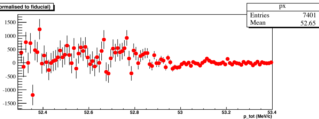
Distribution of Endpoint residuals, BR = 0.000002
