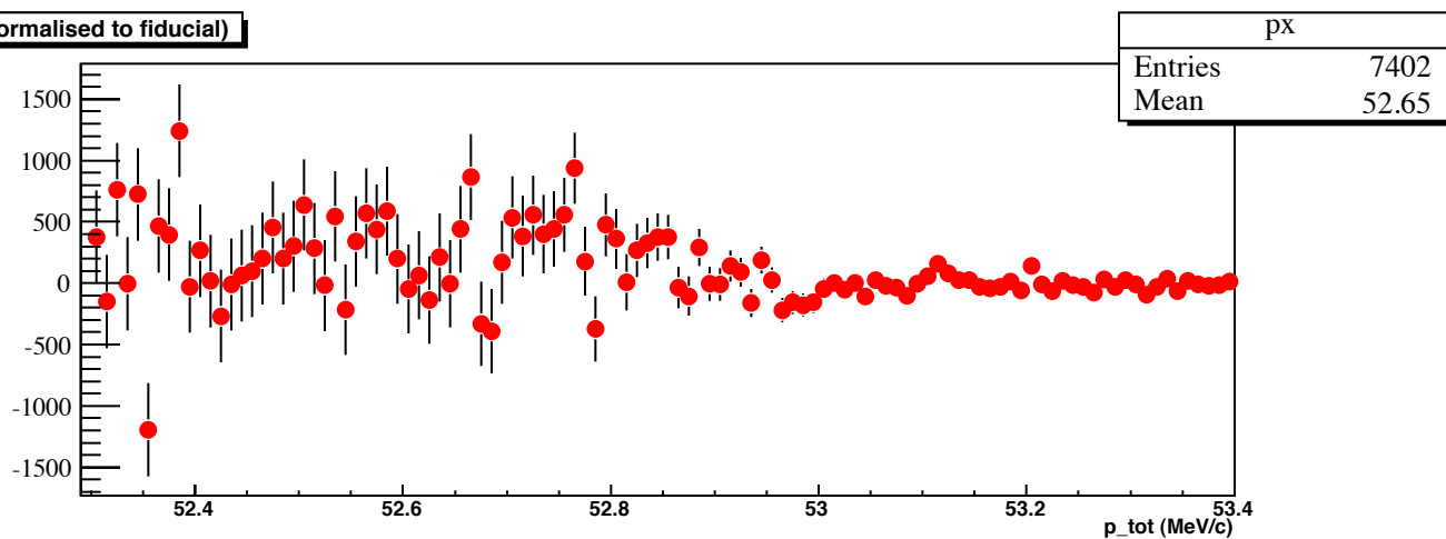
Distribution of Endpoint residuals, BR = 0.000004
