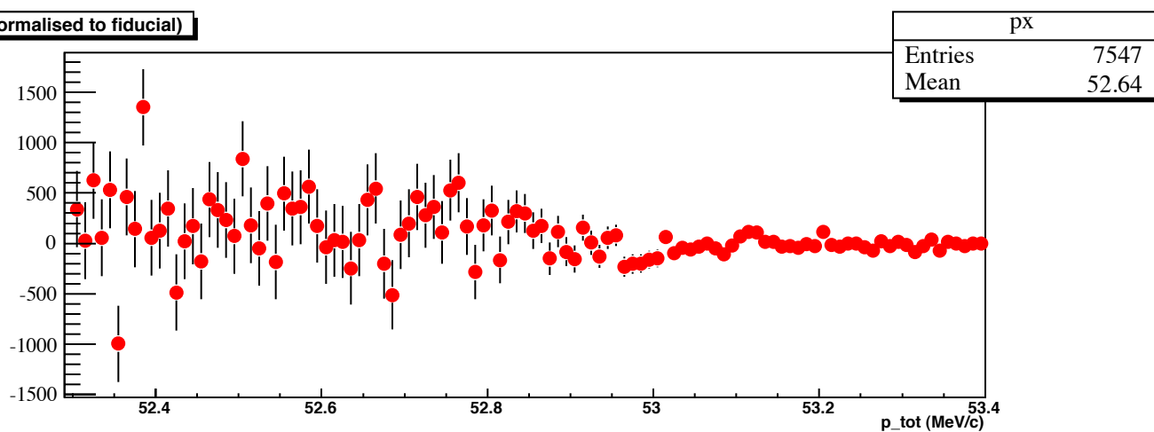
Distribution of Endpoint residuals, BR = 0.000063
