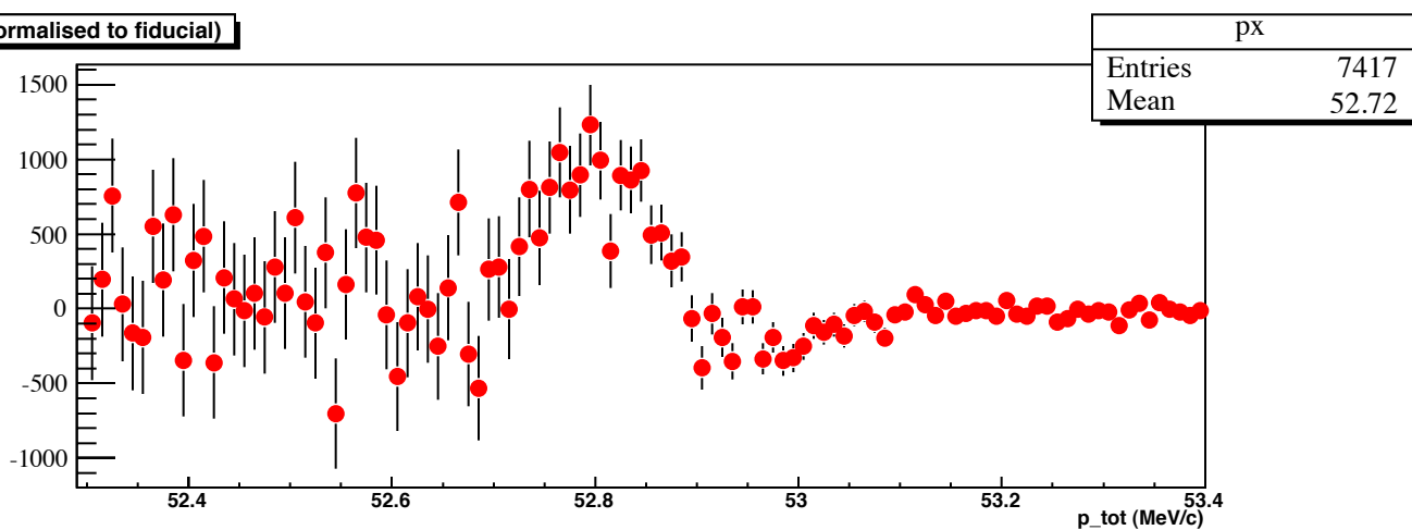
Distribution of Endpoint residuals, BR = 0.000500
