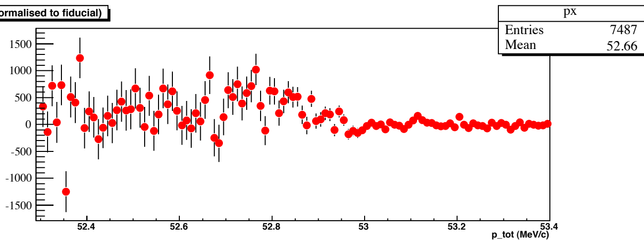
Distribution of Endpoint residuals, BR = 0.000031
