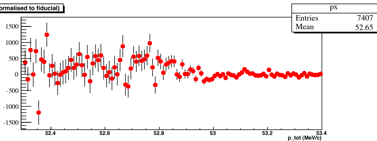
Distribution of Endpoint residuals, BR = 0.000008
