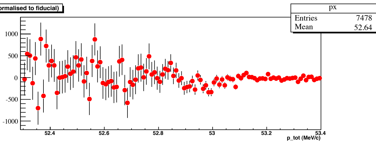
Distribution of Endpoint residuals, BR = 0.000250
