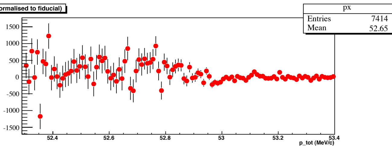
Distribution of Endpoint residuals, BR = 0.000001
