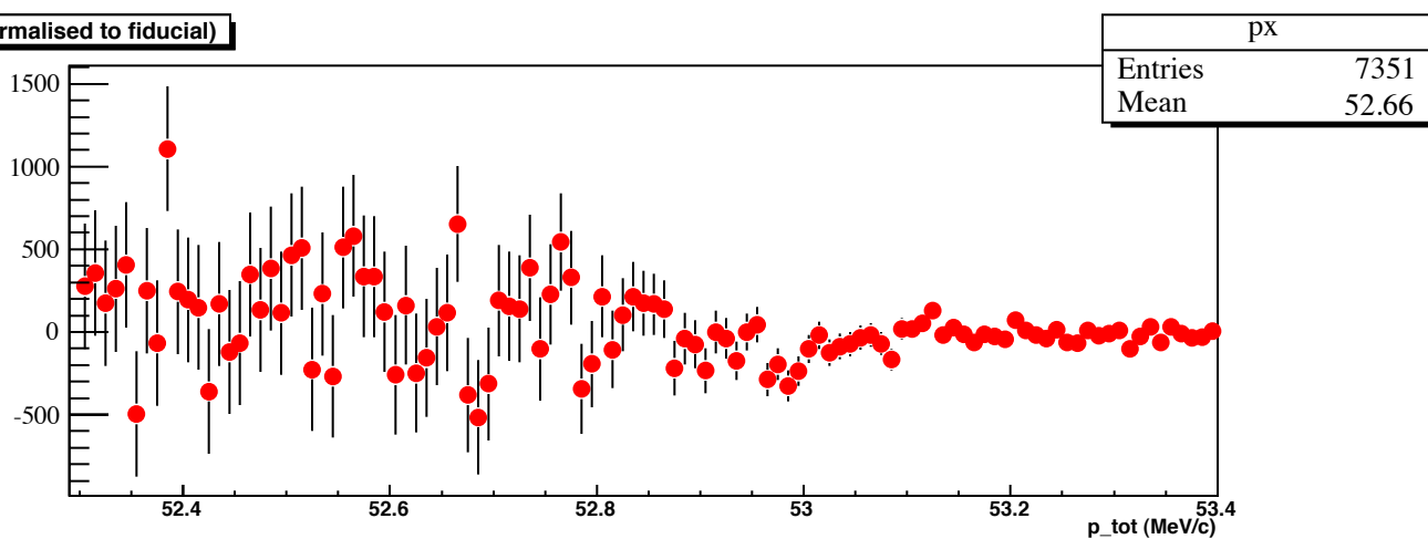
Distribution of Endpoint residuals, BR = 0.000125
