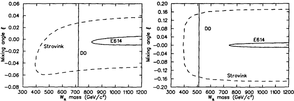
Figure 2. Current and proposed 95% CL limits on W_R mass vs. mixing angle. The curves in the left figure are calculated assuming that the left- and the right-handed CKM matrices are identical. The curves in the right figure make no assumptions on the right-handed CKM matrix. Solid vertical line: W_R mass limit from D0[3]. Solid curve: allowed region from E614 under the same assumptions. Dashed curve: allowed region from Jodidio et al.[2]
