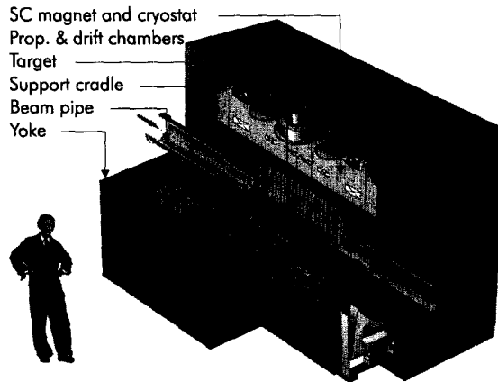
Figure 1. The E614 Spectrometer.
