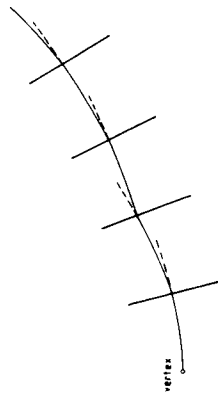
Fig. 1. Particle trajectory in a magnetic field with scattering in the detector planes of a spectrometer.
