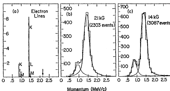
FIG. 4. Conversion-electron spectra. (a) Electron lines (see Table I). Arrow indicates mean momentum of electrons from the 1.7-MeV transition. (b,c) Histograms show events per 0.1 MeV/c in conversion-electron spectra. Solid curves are individual peaks and dashed curves are total spectra as obtained by fitting Eq. (4) to histograms.
