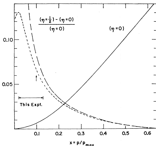
FIG. 1. Sensitivity of the decay spectrum to \eta . Solid line shows \mu^+ decay spectrum for \eta=0 . Long dashed line shows fractional change in spectrum before radiative corrections when \eta is varied from 0 to \frac{1}{2} . Short dashed line shows same change after radiative corrections. Arrow shows mean momentum for this experiment.
