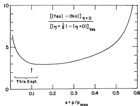
FIG. 2. Effect of the radiative correction. Curve shows ratio of change in spectrum due to radiative corrections to change which occurs when \eta is varied from 0 to \frac{1}{2} . Arrow shows mean momentum for this experiment.
