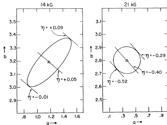
FIG. 5. \eta versus the shape parameters a and b . Ellipses show one standard deviation contours in a and b from fits to 14- and 21-kG Bi 207 data. Triangles show best-fit values. The lines show values of a and b that result in the same fitted values for \eta .
