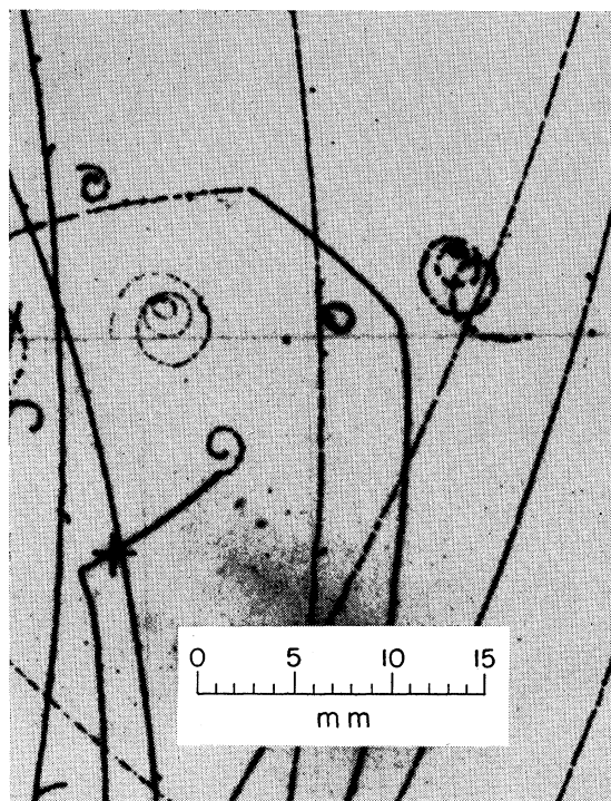
FIG. 3. Sample events. Picture shows two 1.4-MeV/c internal-conversion electrons emerging from the Mylar strip (faint horizontal line), and two \pi^+-\mu^+-e^+ decay chains. One of the positrons has a momentum of 0.7 MeV/c.
